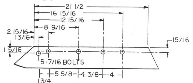
FF18-5RS
