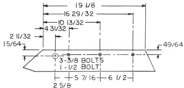
CA16-4RS CA16-4LRS
