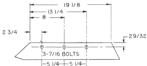
IH14-4RS
