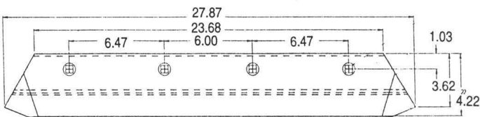
JD24-4RS
