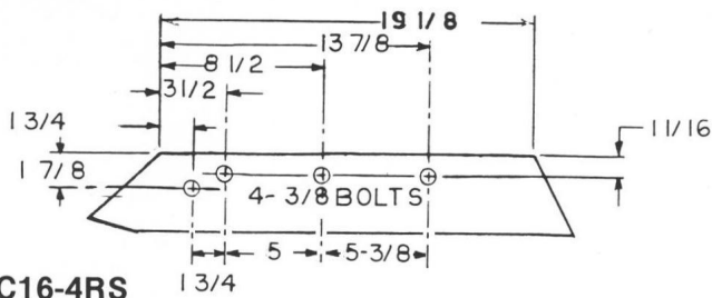
AC16-4RS
